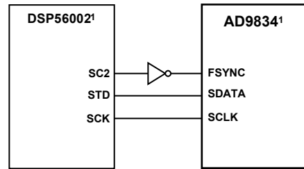
Figure 37. DSP56002 to AD9834 Interface
