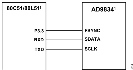
Figure 36. 80C51/80L51 to AD9834 Interface
